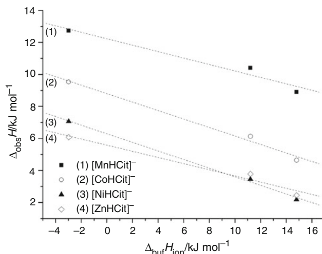
Fig. 2 Plot of \Delta_{\text{obs}}H against \Delta_{\text{ion}}H_{\text{buf}} for the metal–ligand interaction in 10 mM Cacodylate, Pipes and Mes, at a pH of 6, at 298.15 K: (1) \text{Mn}^{2+}/\text{HCit}^{3-} ; (2) \text{Co}^{2+}/\text{HCit}^{3-} ; (3) \text{Ni}^{2+}/\text{HCit}^{3-} ; (4) \text{Zn}^{2+}/\text{HCit}^{3-}
